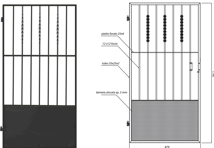
Pedestrian gate \square 31/32" \times 3/32" + \square 31/32" \times 1/4" + \square 15/32" \times 15/32" Fußgängertor \square 25 \times 2 \text{ mm} + \square 25 \times 6 \text{ mm} + \square 12 \times 12 \text{ mm}
